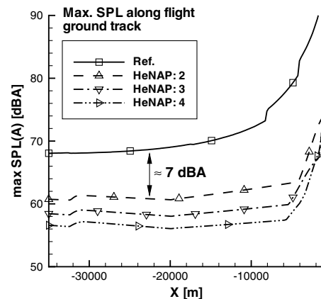
Fig. 4 Predicted maximum SPL_A along flight ground tracks for conventional, medium-range transport aircraft.
